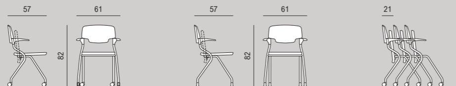
SEDUTA ATTESA RIBALTABILE IMBOTTITA CON BRACCIOLI | PADDED VISITOR CHAIR WITH FOLDING SEAT AND ARMRESTS
