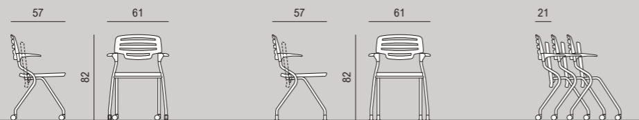
SEDUTA ATTESA RIBALTABILE CON BRACCIOLI | VISITOR CHAIR WITH FOLDING SEAT AND ARMRESTS
