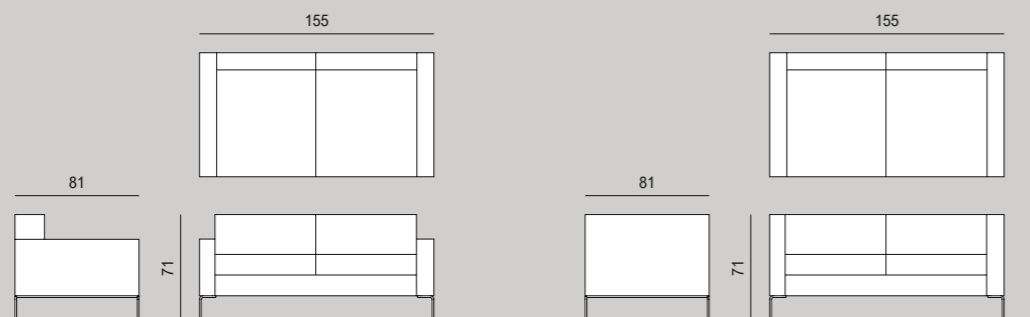
DIVANO 2 POSTI CON BRACCIOLI BASSI E ALTI | 2-SEATER SOFA WITH LOW AND HIGH ARMRESTS
