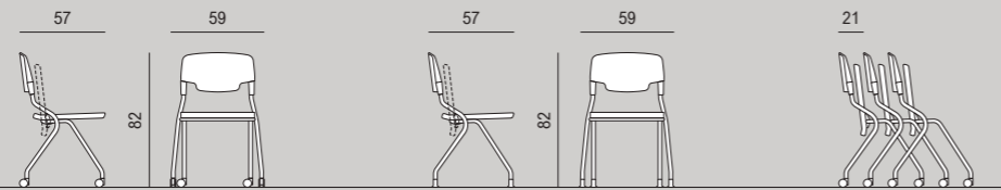
SEDUTA ATTESA RIBALTABILE IMBOTTITA | PADDED VISITOR CHAIR WITH FOLDING SEAT
